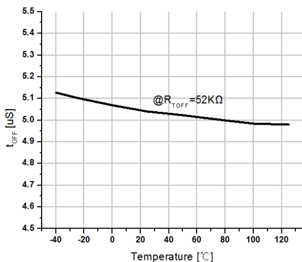
t_{OFF}(R_{TOFF}=52k\Omega) vs. Temp
