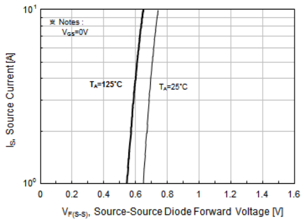
Fig.6 Forward Source to Source Characteristics
