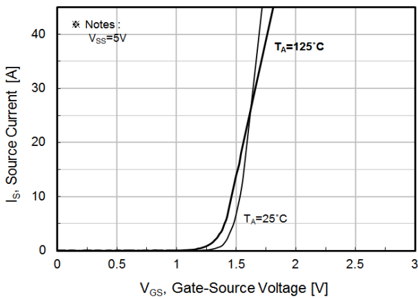
Fig.5 Transfer Characteristics
