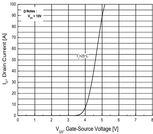
Fig.5 Transfer Characteristics
