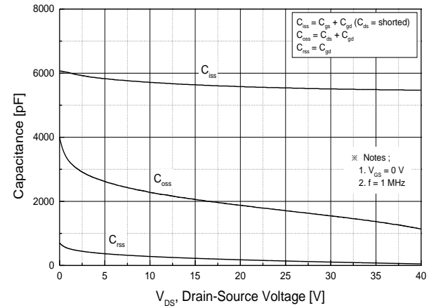
Fig.8 Capacitance Characteristics
