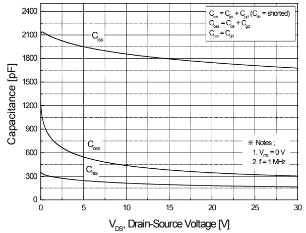
Fig.8 Capacitance Characteristics
