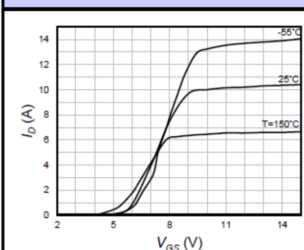
Fig.5 Transfer Characteristics
